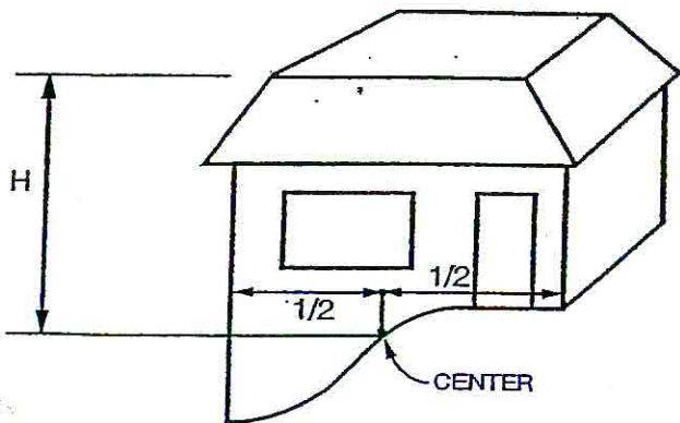
MANSARD ROOF
